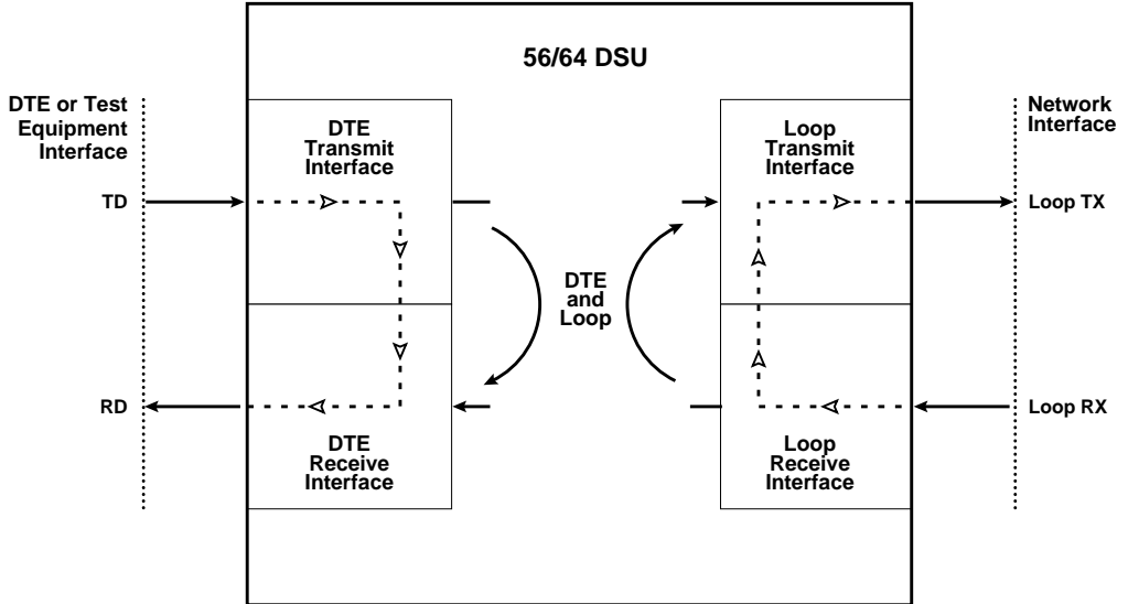
Figure 3-3 DTE and Loop Test Diagram
